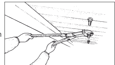
Cut the bolts while avoiding contact with the asbestos cement
